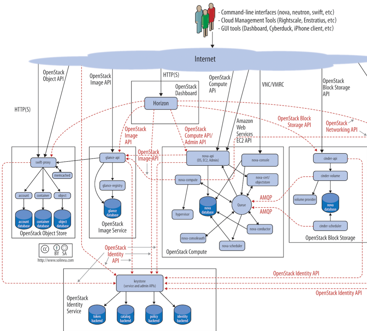
Figure 1. OpenStack Logical Architecture ( http://docs.openstack.org/openstack-ops/content/figures/2/figures/osog_0001.png )
