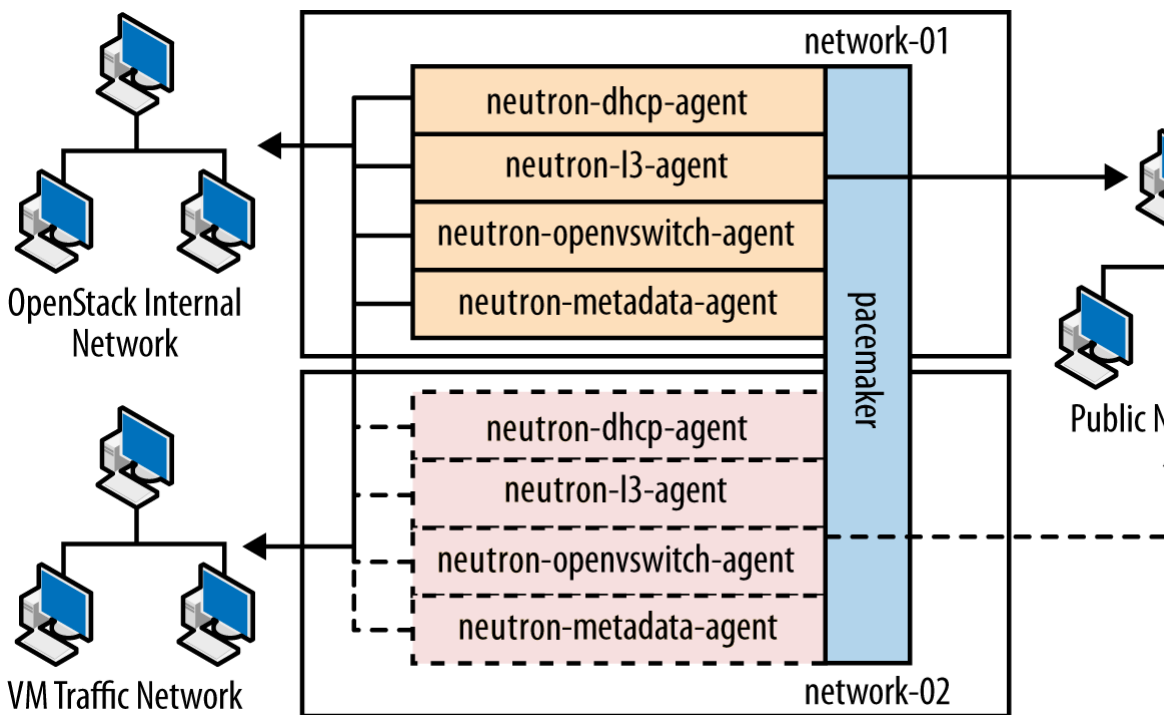
Figure 1.5. Network node
