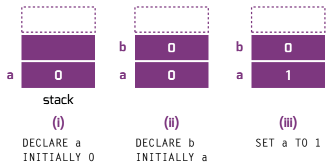
■ Figure 1: integer variable to variable assignment
