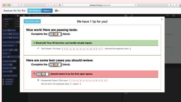
■ The test results for a simple noughts and crosses game: this shows one passing and one incorrect test
