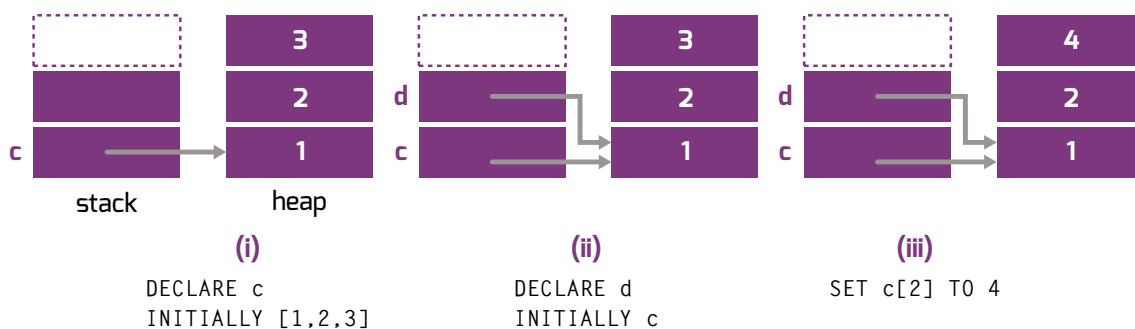
Array variable to variable assignment with address sharing. After assigning a structure type from a source variable to a target variable, changing via the source changes the target
