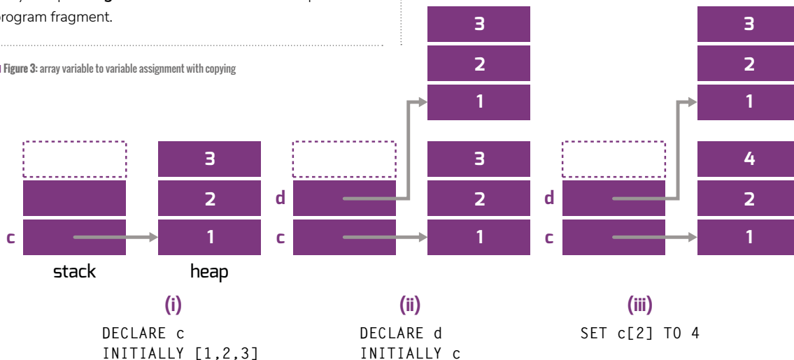
Array variable to variable assignment with copying. After assigning a structure type from a source variable to a target variable, changing via the source doesn't change the target
