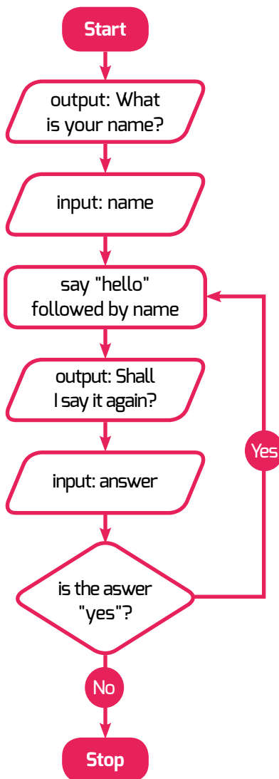
Figure 2: the same program as a flowchart - note the identical structure
