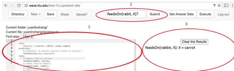
Figure 1: Screenshot of onlineSPARC
